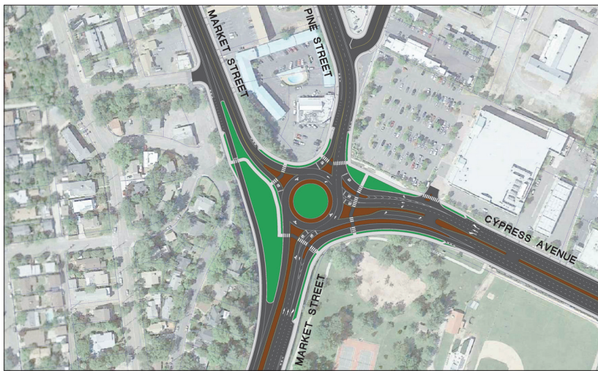
Figure 3 – Example of a Modern Roundabout at Cypress/Pine/Market Street Intersection
