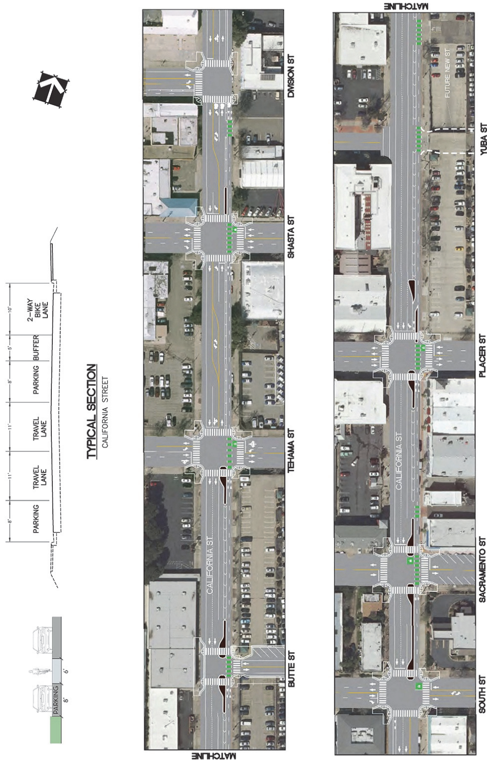
Figure I3 – Conceptual Plan View & Section for Protected Bike Lanes on California Street
