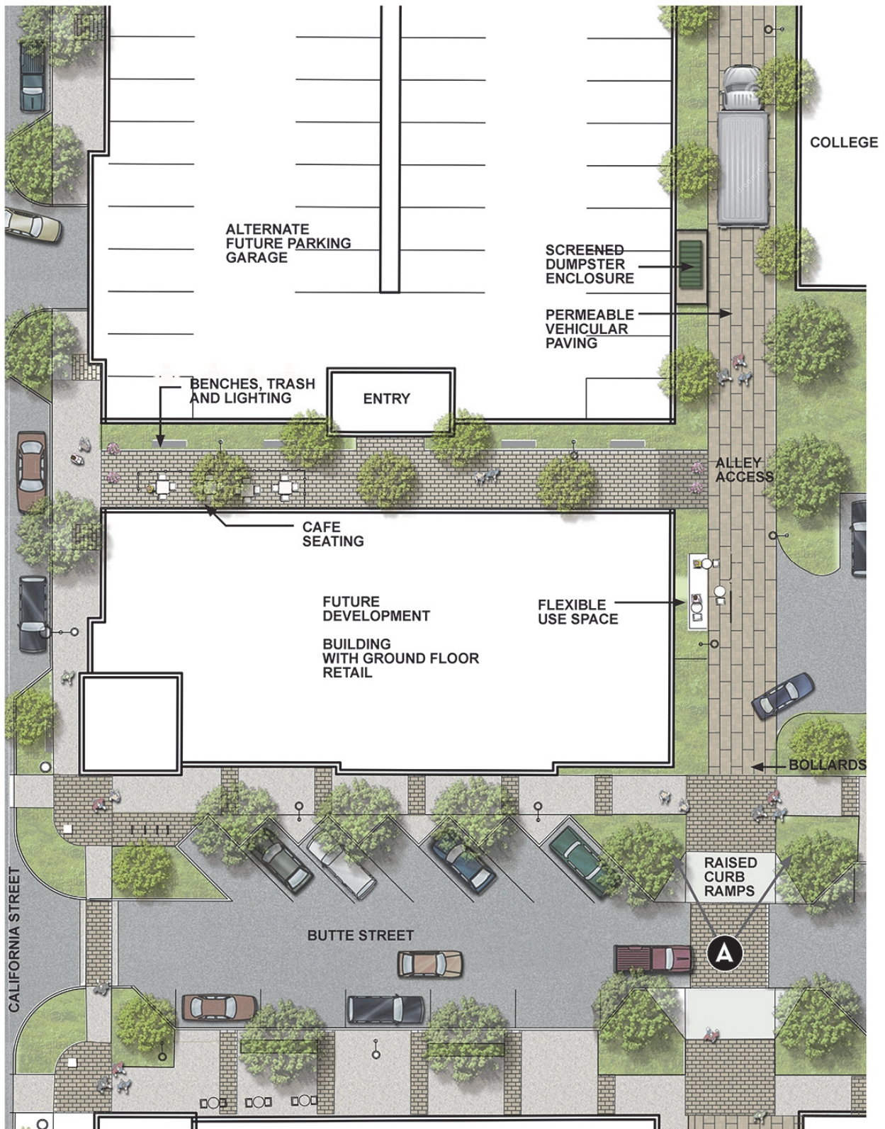
Figure H8 – Conceptual Site Plan with Design Elements along the California-Market Alley
