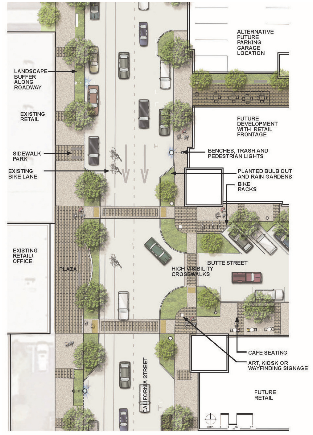
Figure 6 – Typical Design Elements to Provide a Quality Pedestrian Environment
