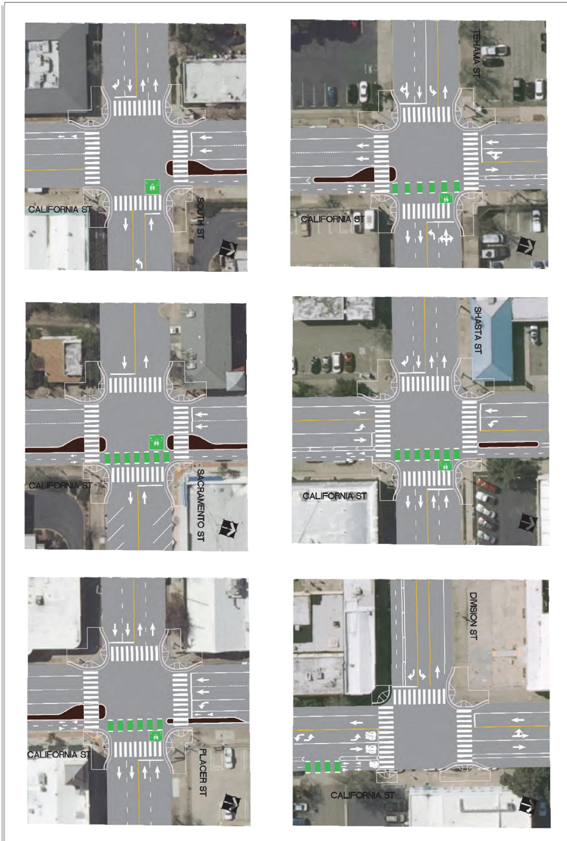
Figure I2 – Conceptual Illustrations for Protected Bike Lanes on California Street
