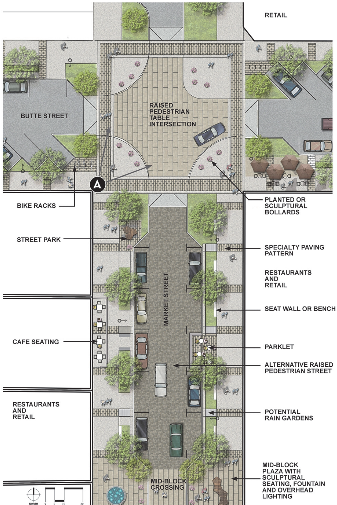
Figure H7 – Conceptual Market Street Promenade Site Plan
