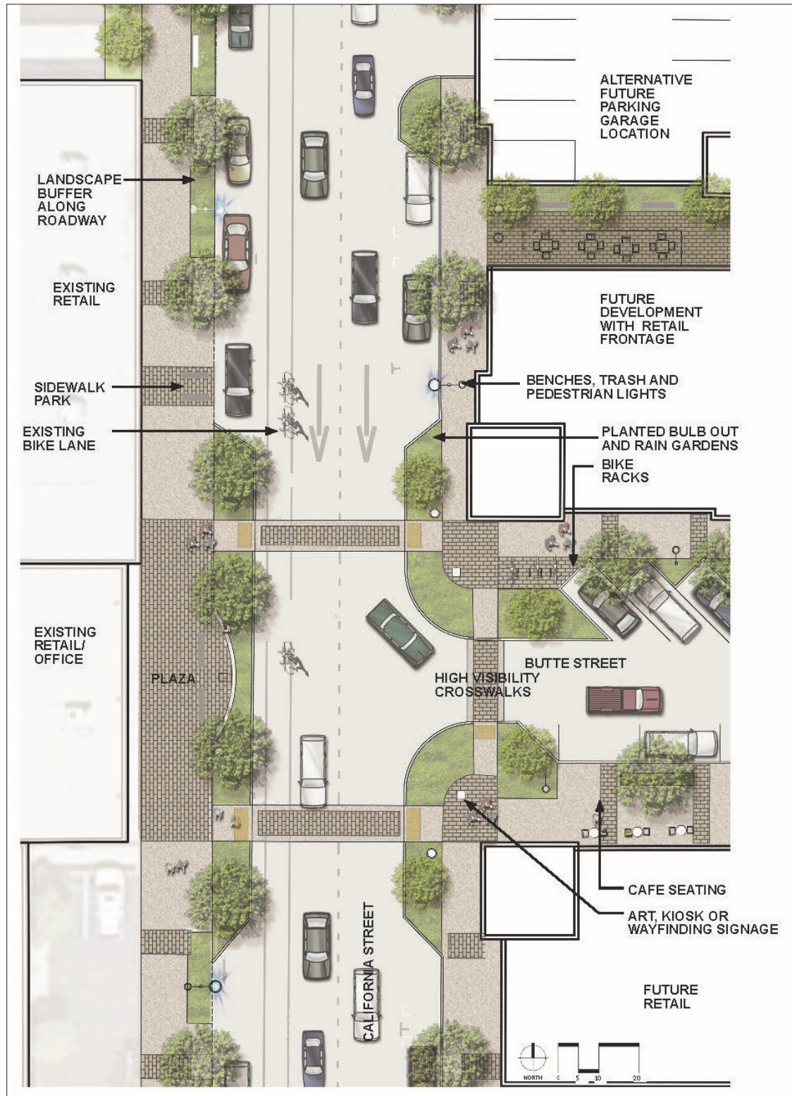
Figure H16 – Typical Design Elements to Provide a Quality Pedestrian Environment (NOTE: A protected bike lane is recommended in addition to what is shown above)
