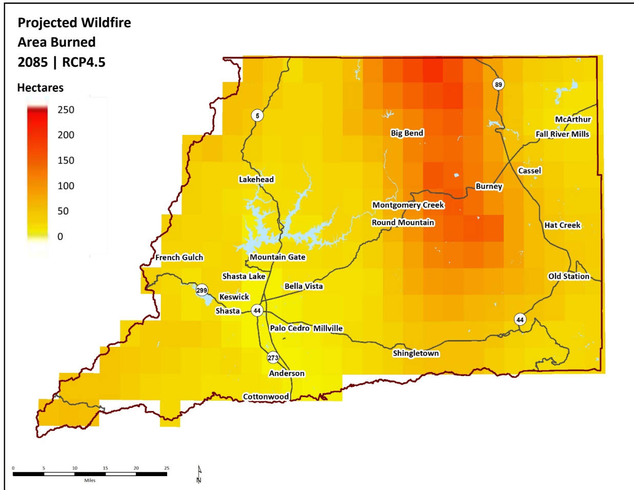
Figure 147. Average annual area burned in 2085, RCP4.5.
