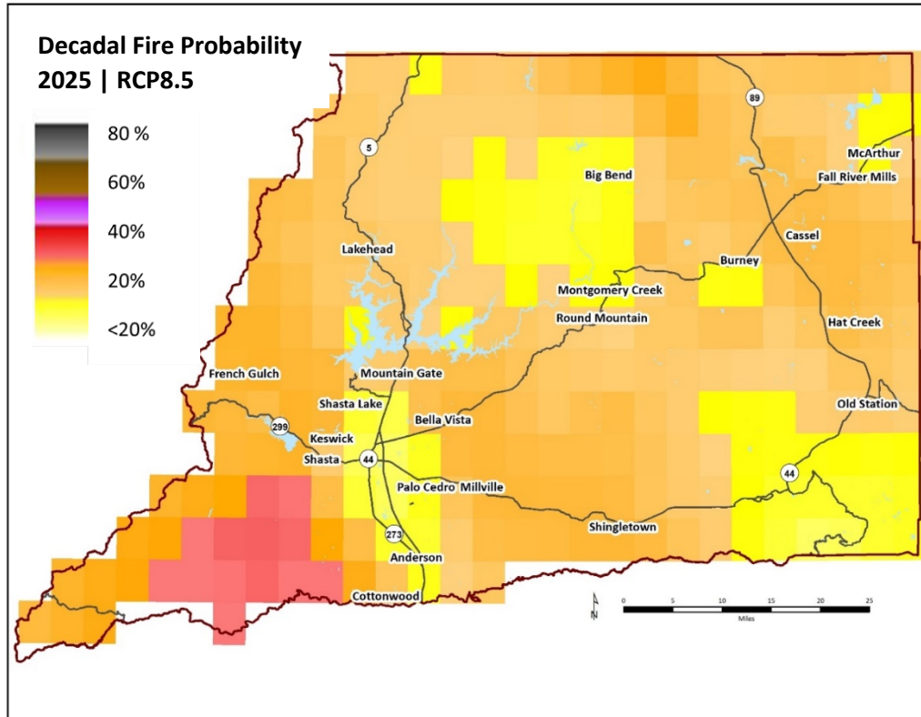
Figure 35. Decadal Fire Probability in 2025, RCP8.5.
