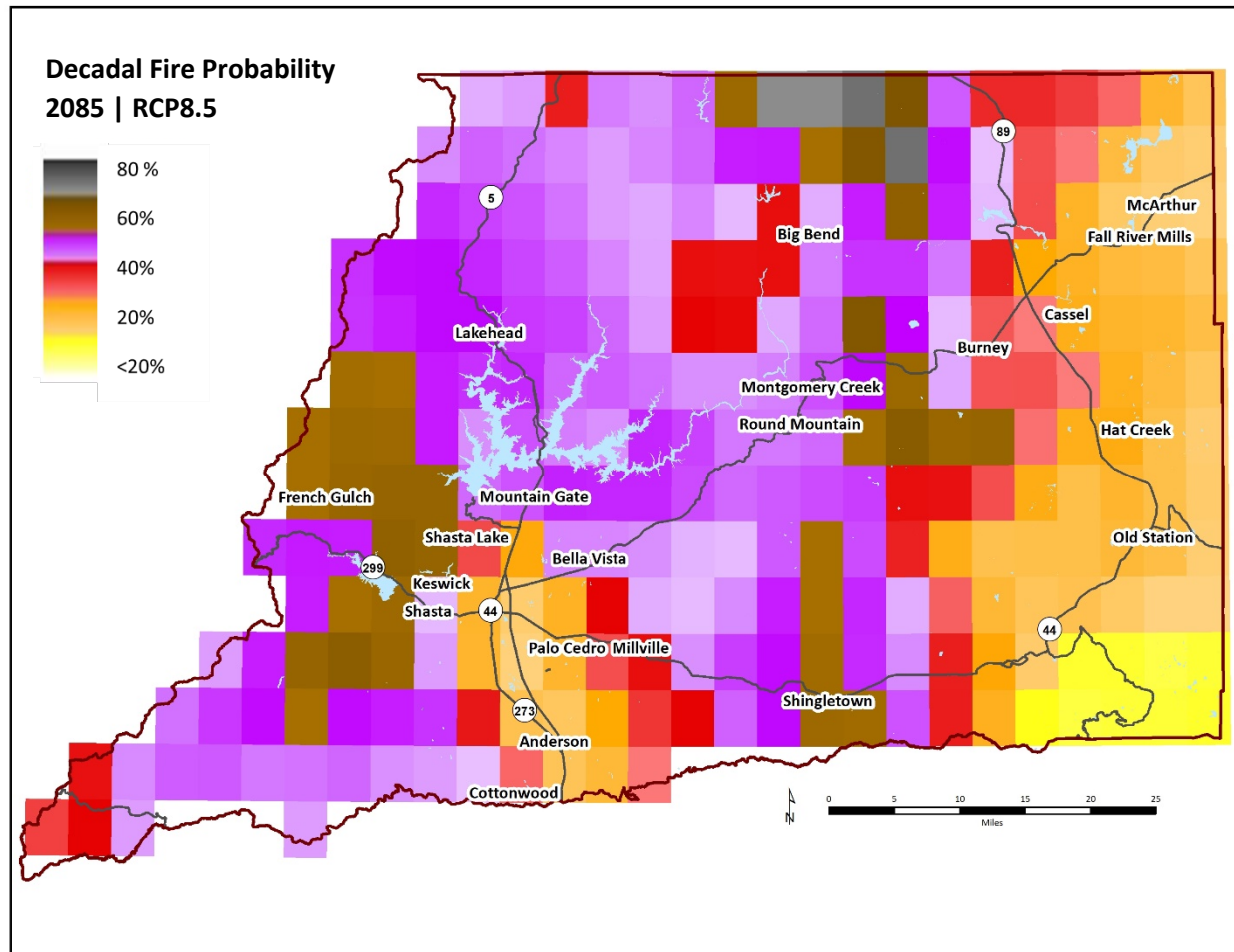
Figure 37. Decadal Fire Probability in 2085, RCP8.5.
