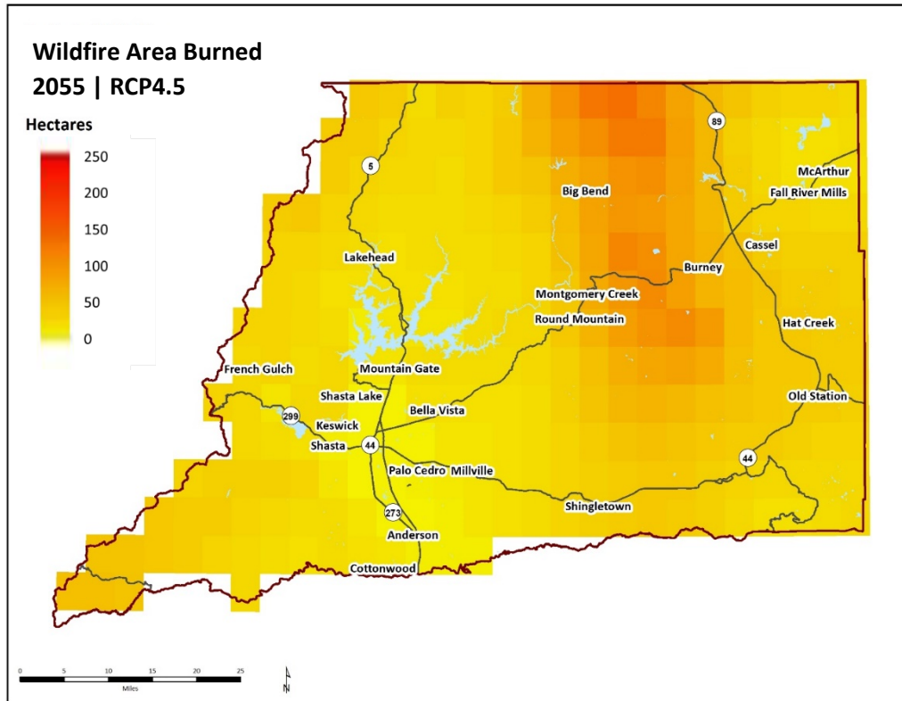
Figure 46. Average annual area burned in 2055, RCP4.5.
