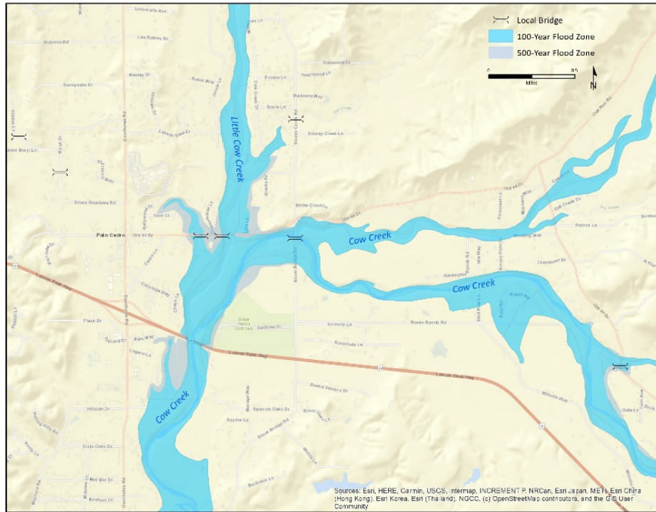
Figure 69. Floodplains in Palo Cedro.
