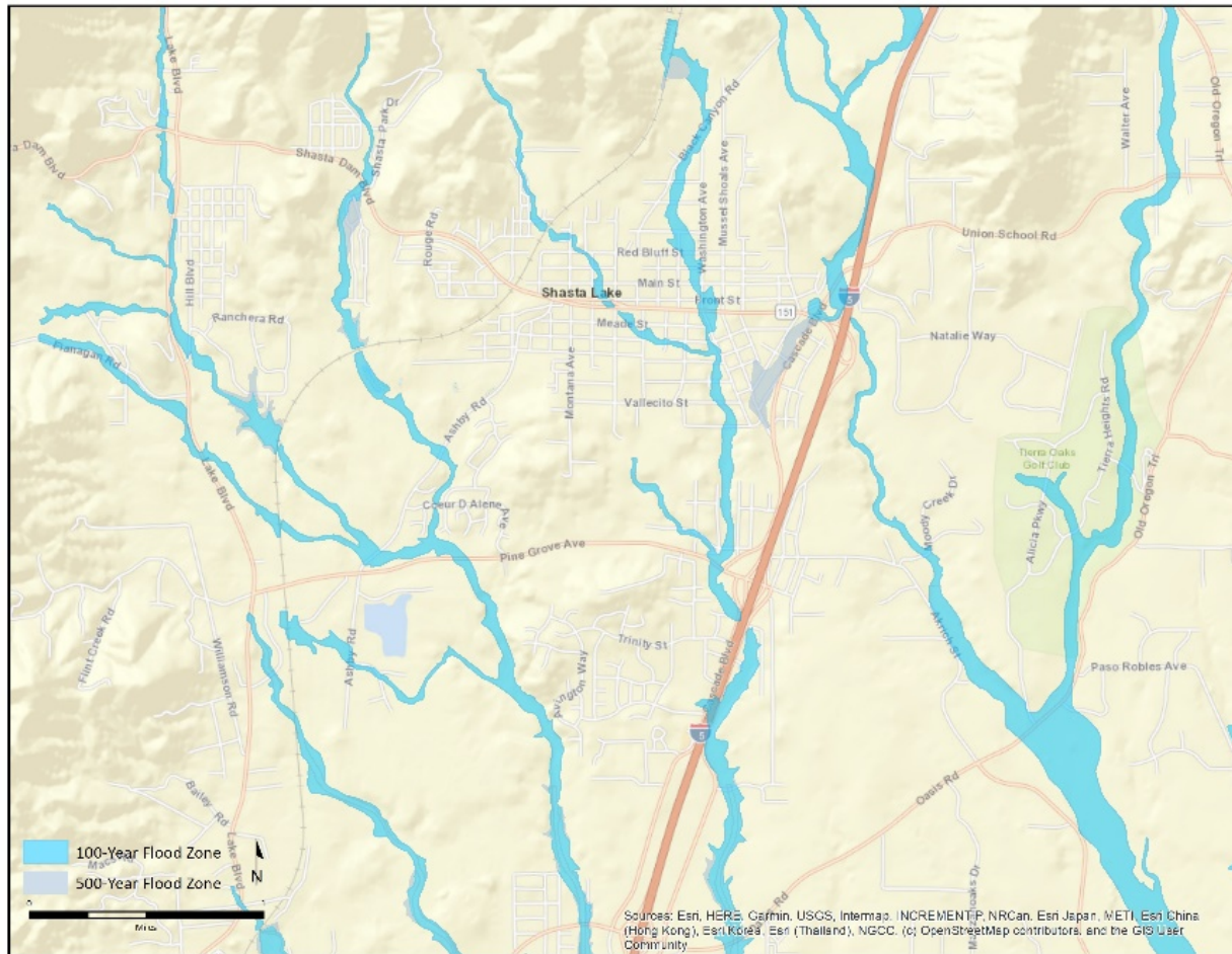
Figure 66. Tributaries and flooding exposure in the City of Shasta Lake.
