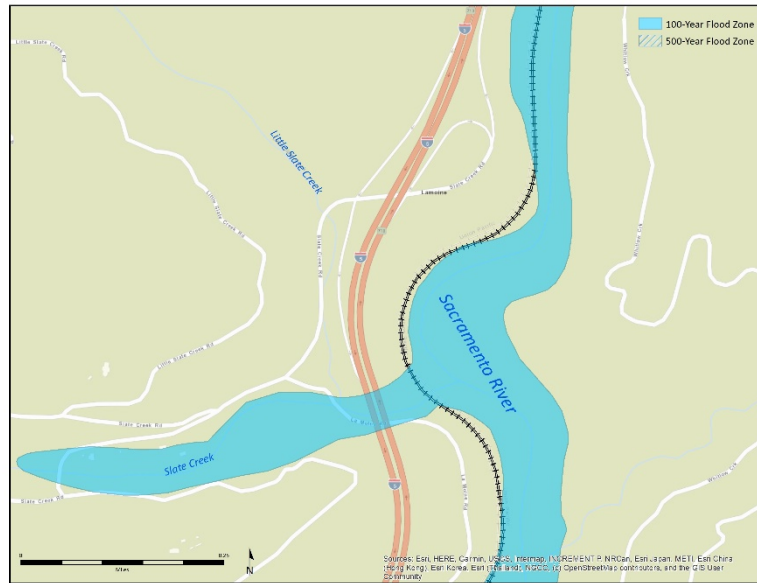
Figure 71. Flooding exposure of the Union Pacific Railroad in the Sacramento River Canyon, near Lamoine.
