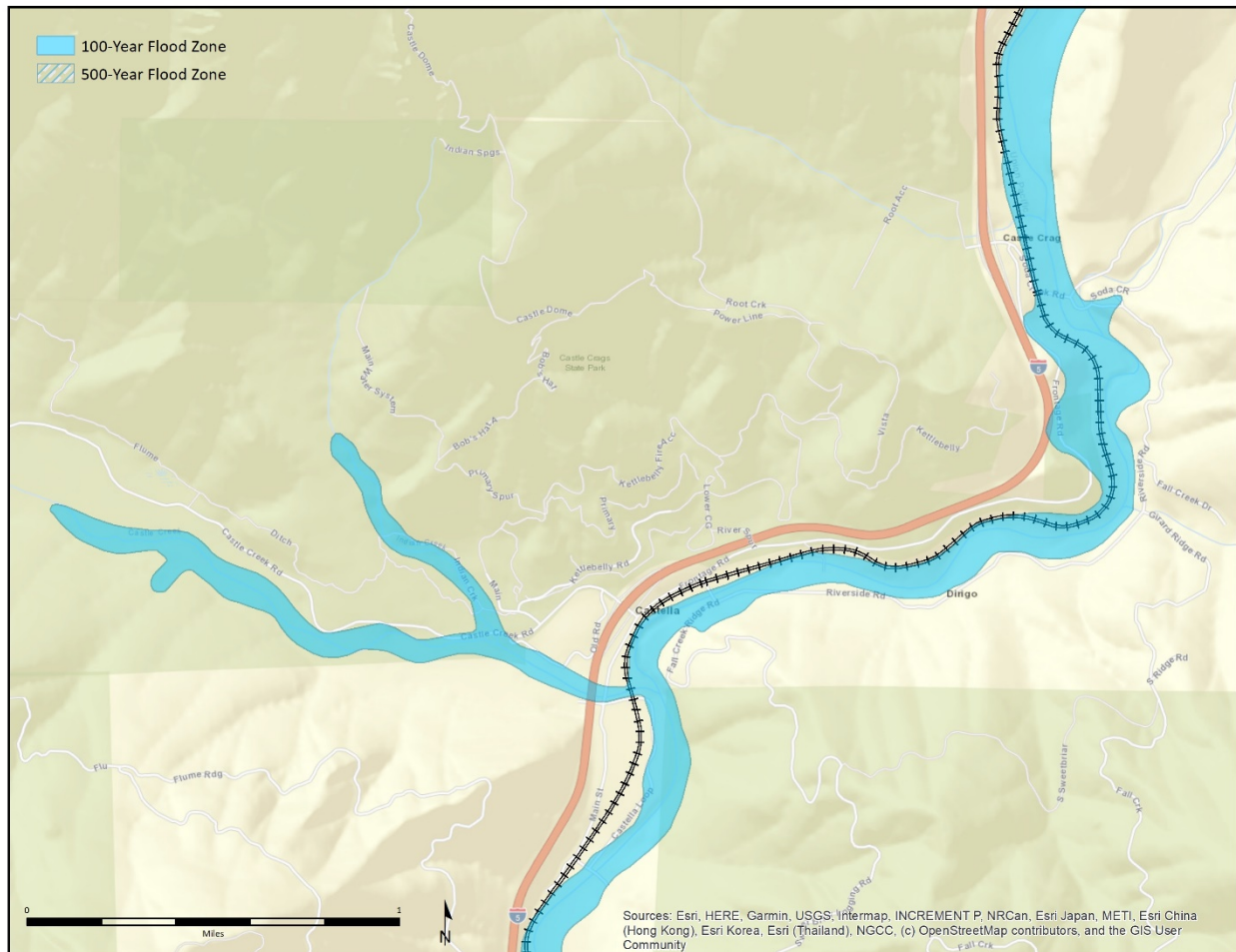
Figure 73. Flooding exposure of the Union Pacific Railroad in the Sacramento River Canyon, near Castle Crag State Park.
