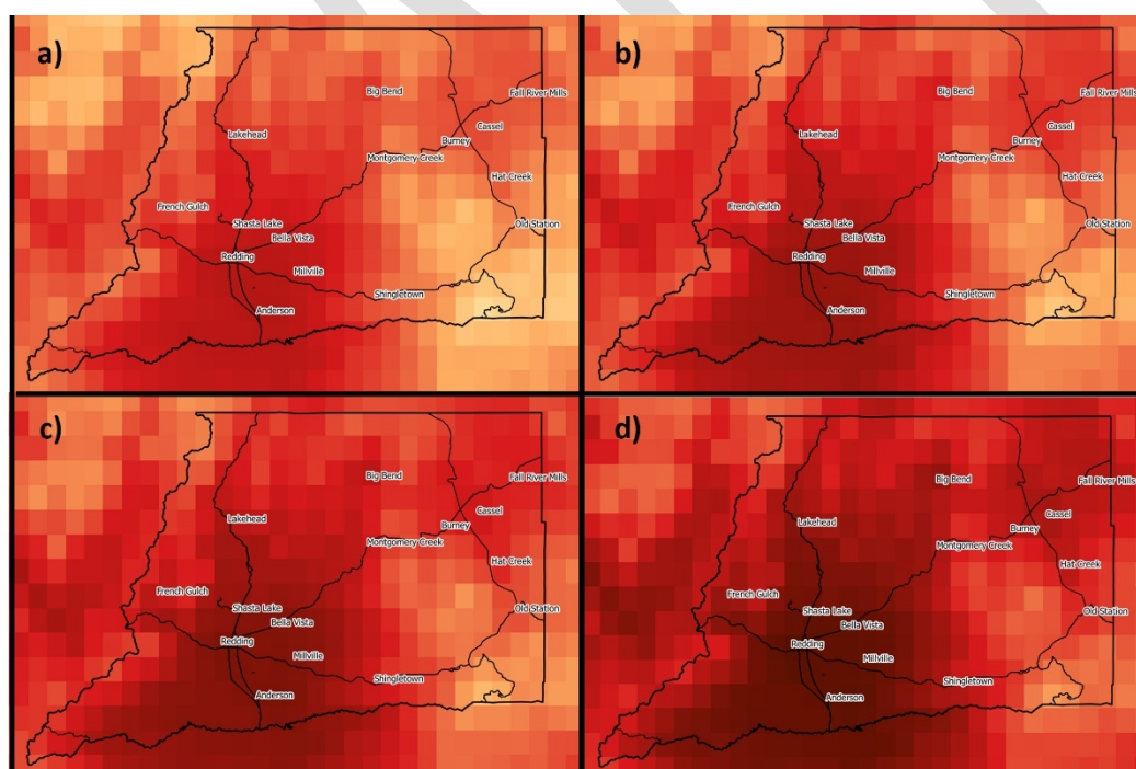
Figure 9. Historical and projected heat wave temperatures in the Shasta Region in an unconstrained emissions scenario (RCP8.5).
