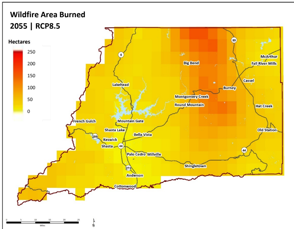
Figure 43. Average annual area burned in 2055, RCP8.5.
