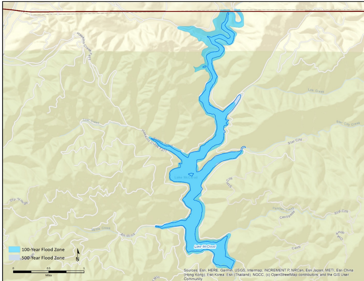
Figure 80. Flood hazards around Lake McCloud.
