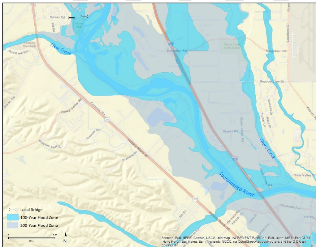
Figure 64. Flooding exposure in along Highway 273, north of Anderson.
