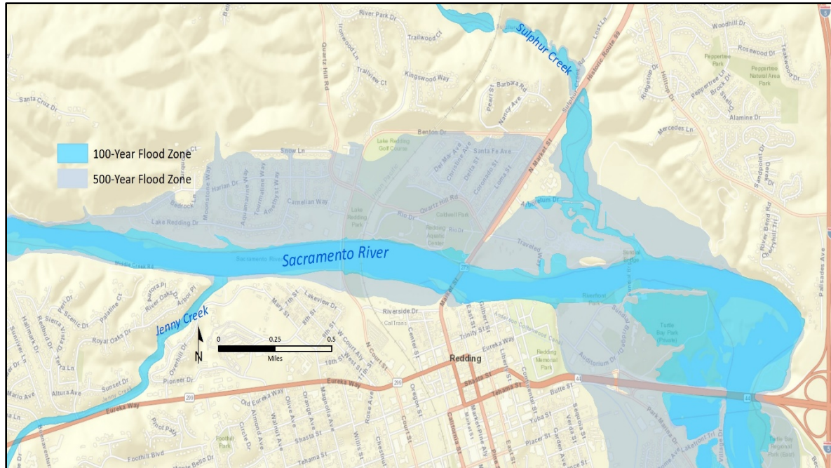
Figure 61. Flooding exposure in Central Redding, north of Highway 299.
