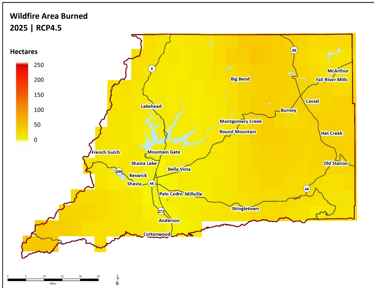
Figure 45. Average annual area burned in 2025, RCP4.5.
