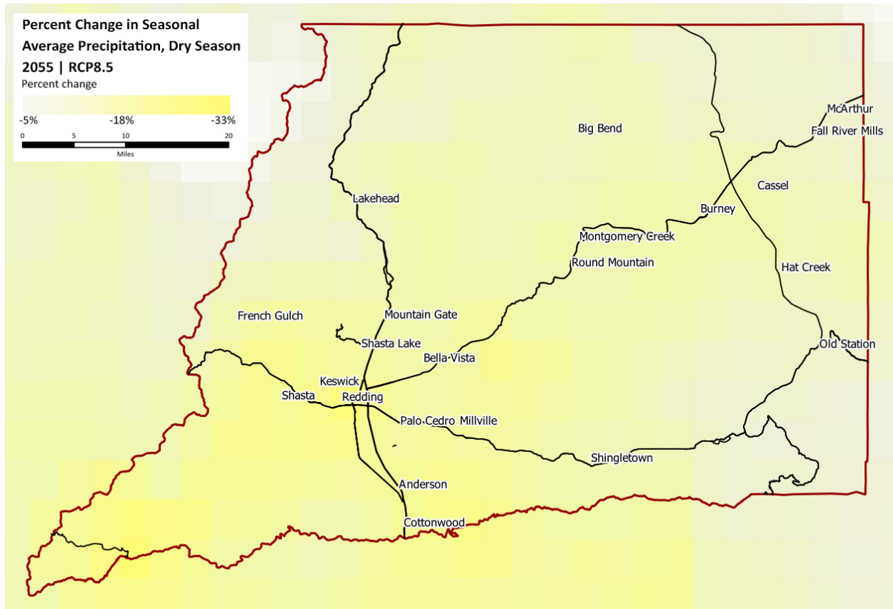
Figure 113. Percent change in dry season precipitation, 2055 RCP8.5.
