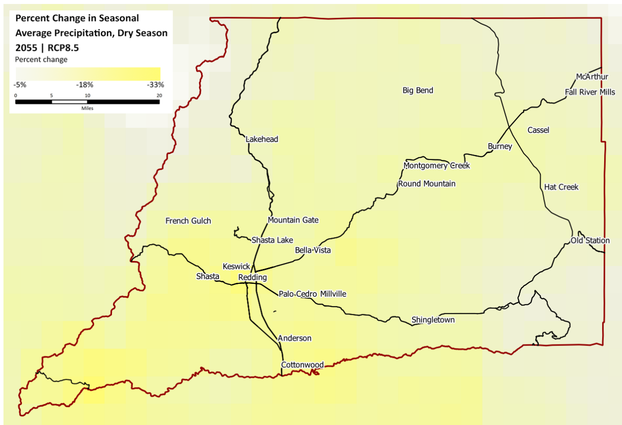
Figure 18. Percent change in dry season precipitation, 2055 RCP8.5.
