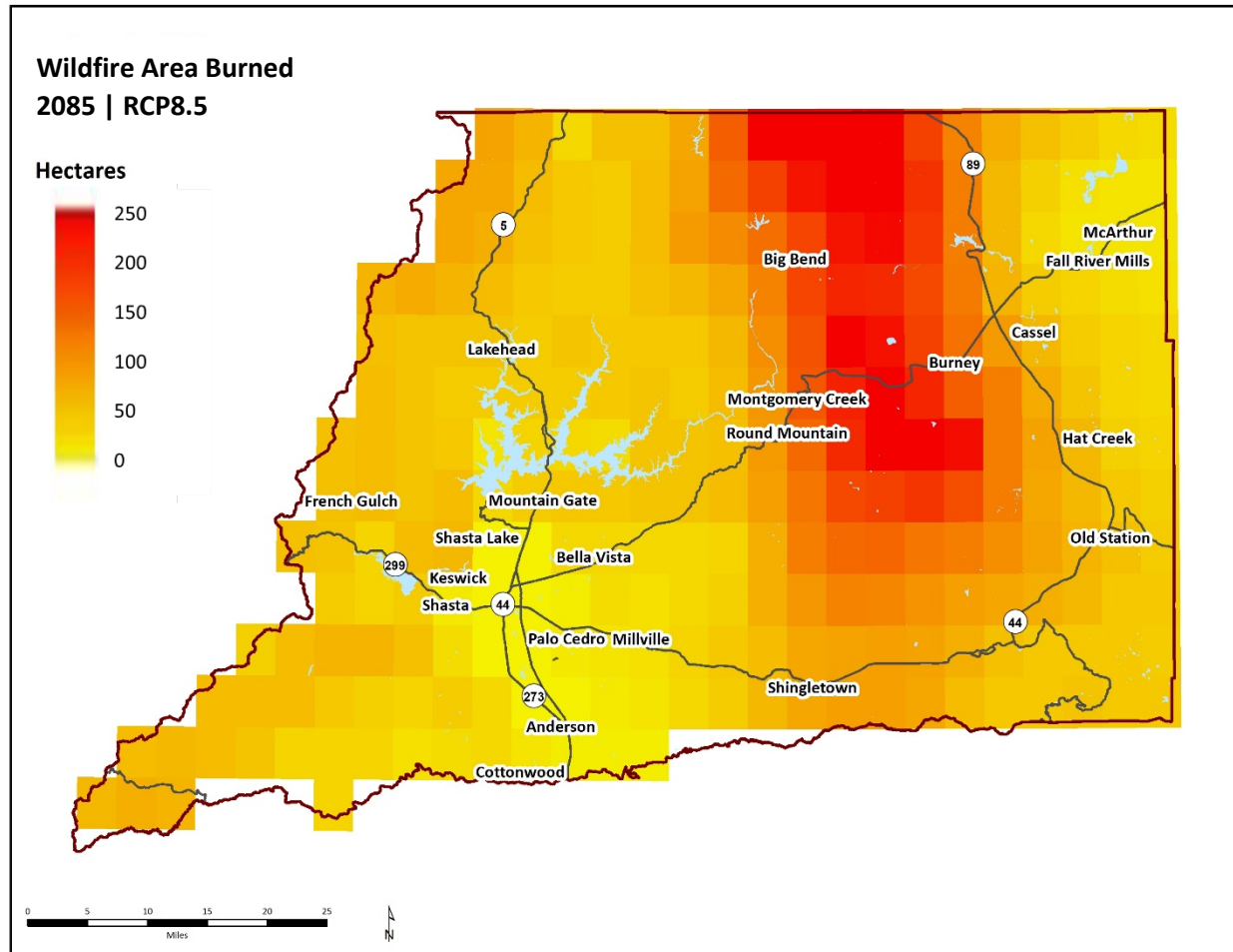
Figure 44. Average annual area burned in 2085, RCP8.5.
