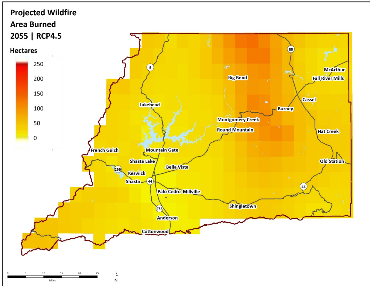
Figure 146. Average annual area burned in 2055, RCP4.5.
