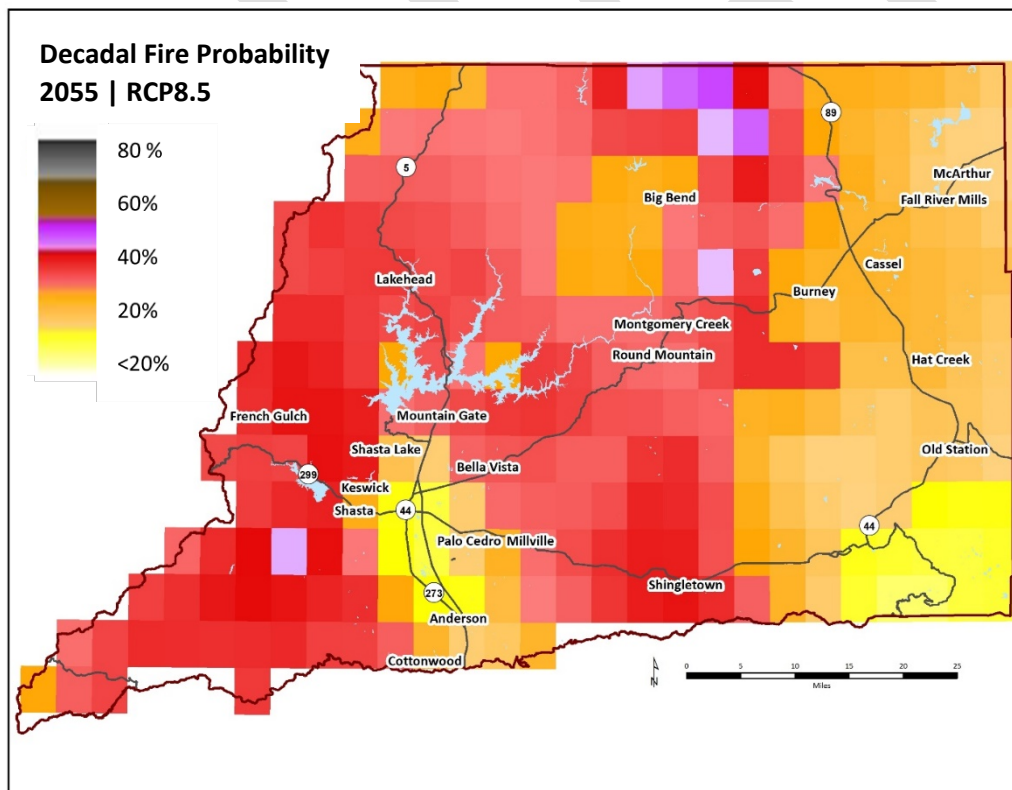
Figure 36. Decadal Fire Probability in 2055, RCP8.5.
