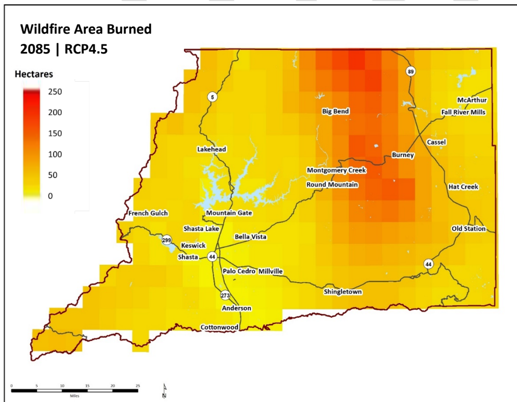
Figure 47. Average annual area burned in 2085, RCP4.5.
