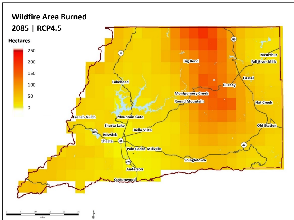
Figure 46. Average annual area burned in 2085, RCP4.5.
